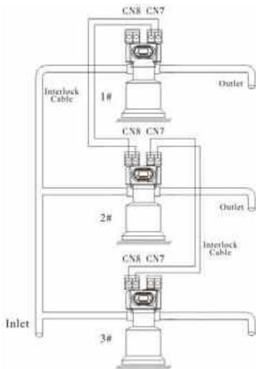
Figure 3-12 Interlock system
